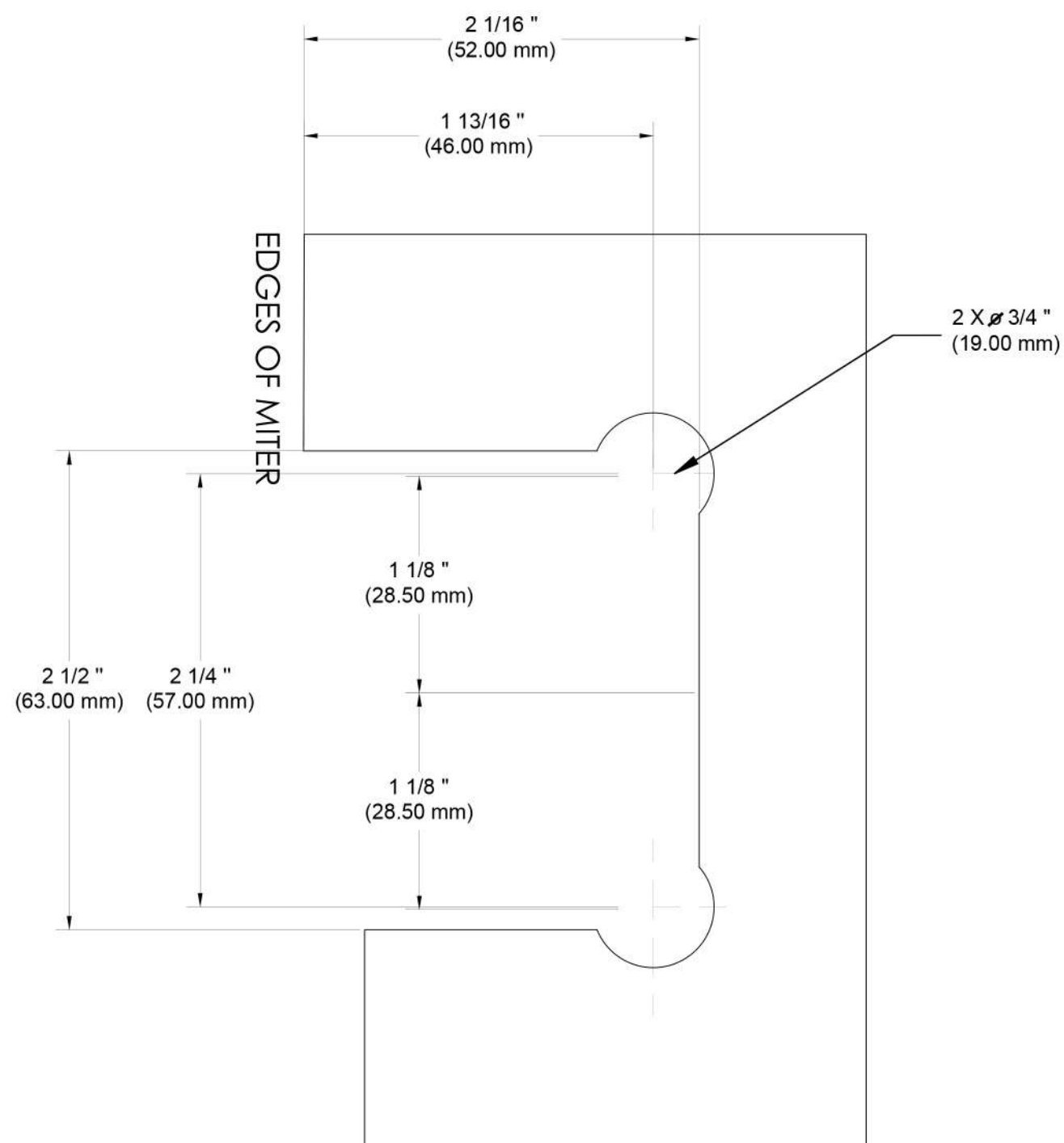
MITERED FIXED PANEL TEMPLATE
