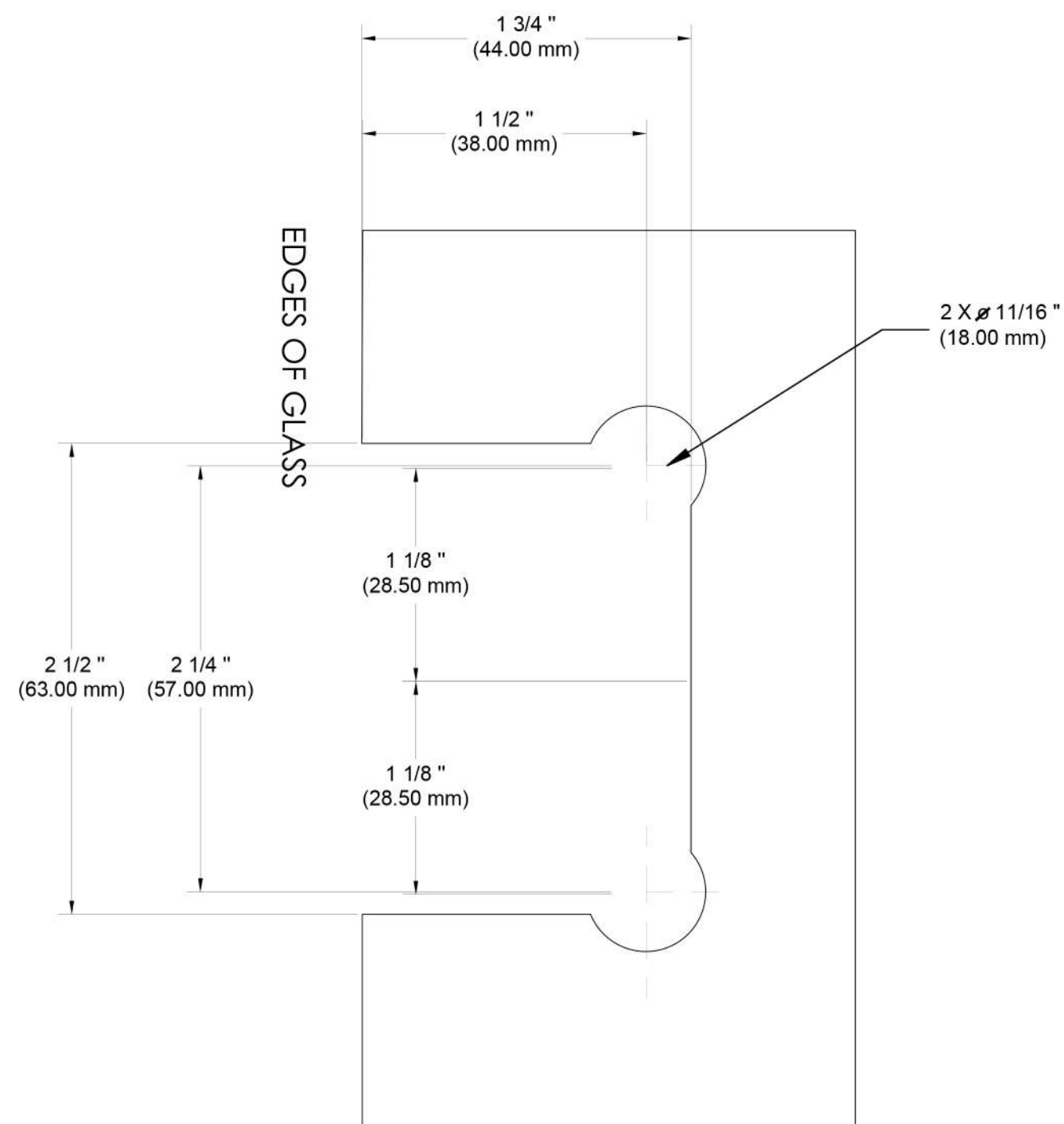
SQUARE CUT TEMPLATE
